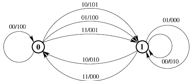
Fig. 3. A rate 2:3 sliding-block decodable encoder for the (1, \infty) constraint.
