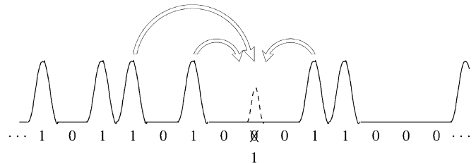
Fig. 1. Model of ghost-pulse formation due to the interaction of three pulses.
