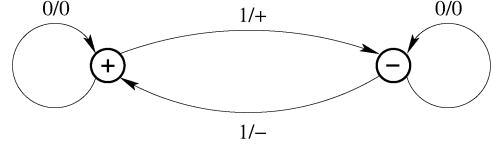
Fig. 5. Simple rate 1:1 two-state encoder for the TGP(1) constraint.
